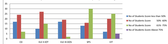
Subject wise Number of students per percentage score band
