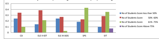
Subject wise percentage of students per percentage score band
