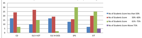
Subject wise Number of students per percentage score band
