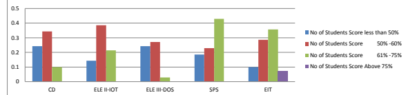
Subject wise percentage of students per percentage score band
